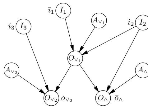
Figure 3: Bayesian diagnostic system corresponding to the circuit in Figure 1.
