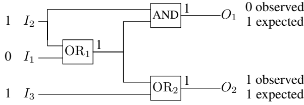
Figure 1: Example of a circuit.
