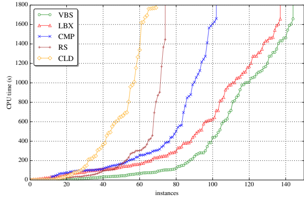
Figure 2: Running times from maxsat instances.
