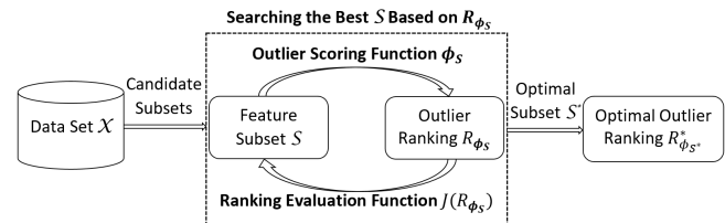
Figure 1: The Proposed WrapperOD Framework
