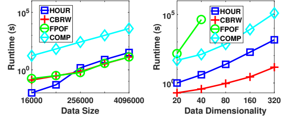
Figure 3: Scale-up Test w.r.t. Data Size and Dimensionality. FPOF runs out of memory when dimensionality reaches 80.
