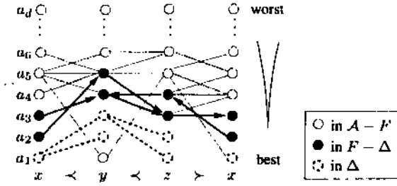
Figure 3: Example for a stable activation.
