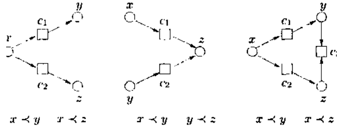
Figure 1: Directed constraint graphs.
