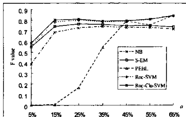
Figure 5 Average results for all a settings
