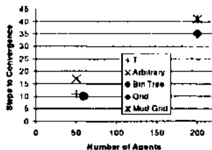
Figure 6: Steps to convergence for the five graphs
