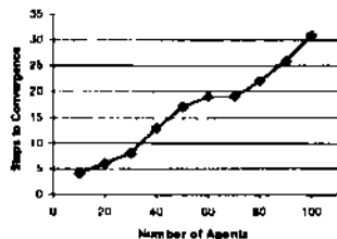
Figure 7: Steps to convergence for the arbitrary graph
