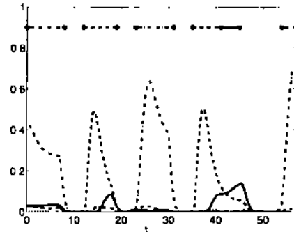
Figure 3: Evolution of the probability for a person of being in different resting areas over the time.
