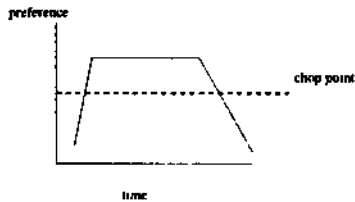
Figure 1: "Chopping" a semi-convex function
