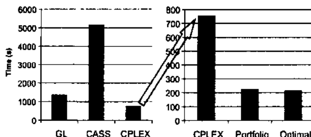
Figure 1: Algorithm and Portfolio Runtimes
