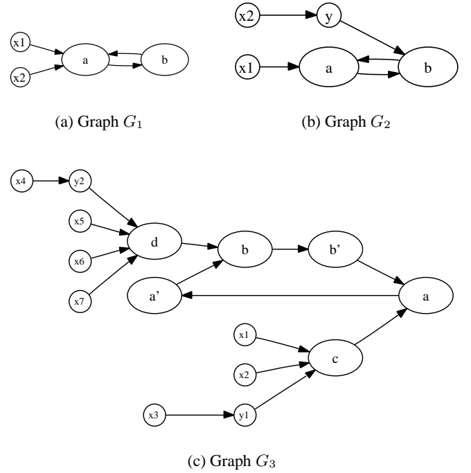
Figure 4: Graphs from the proof of proposition 6.1
