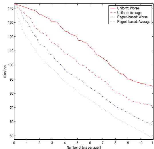
Figure 2: Worst case and expected \epsilon , as a function of the number of bits used per agent. Averaged over 30 runs.
