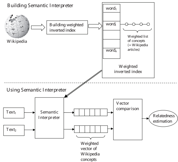
Figure 1: Semantic interpreter
