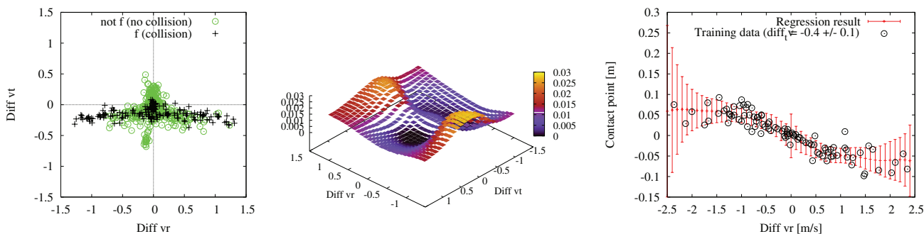
Figure 2: The collision event training set where two feature values are mapped to class instances (left), the learned class probabilities \pi_f(F_t) using Gaussian process classification (middle), and the learned regression model for the collision parameters visualized by a cut through the 2-dimensional pdf that maps velocity deviations to contact points for a collision (right).
