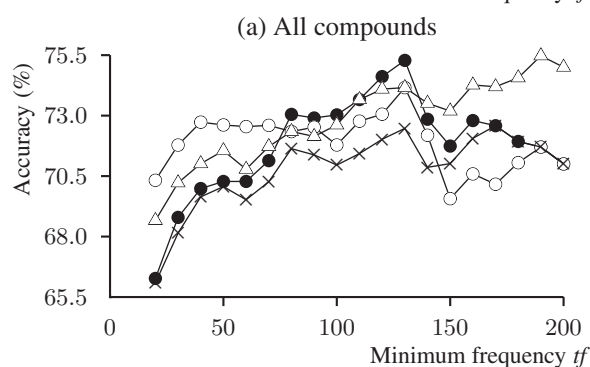
Figure 1: Accuracy of MCS tests as a function of minimum frequency of compounds
