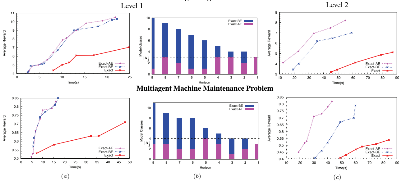
Figure 6: Performance profiles for the multiagent tiger and MM problems generated by executing the solutions obtained using different exact approaches. (a,b) Profiles for level 1 I-DIDs. Notice that Exact-AE maintains less classes at larger horizons in comparison to Exact-BE and never more than |A_j| . (c) Solving level 2 I-DIDs reveals the efficiency facilitated by aggregation using action equivalence.
