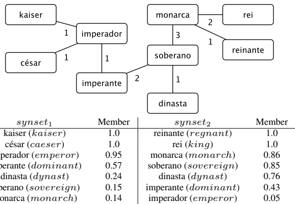
Figure 1: Weighted synonymy graph and resulting synsets
