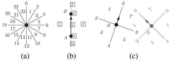
Figure 1: (a) STAR_4 relations. (b) The nine directional LR relations. (c) Relation A \overset{\perp}{L}_7 B in OPRA_2 .
