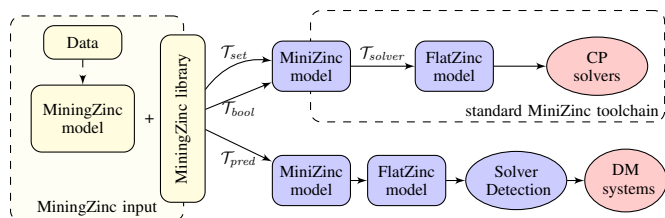
Figure 1: Overview of the MiningZinc toolchain
