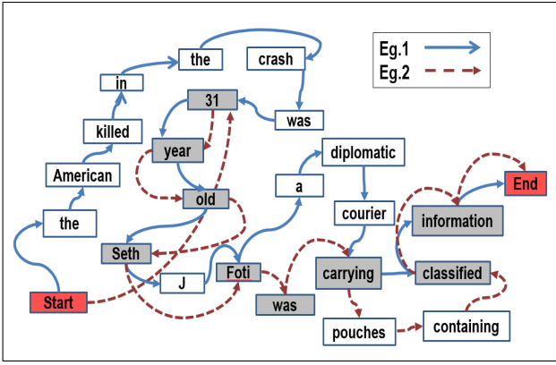
Figure 2: Word-graph generation from sentences.
