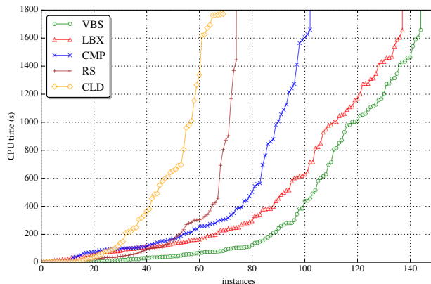
Figure 2: Running times from maxsat instances.
