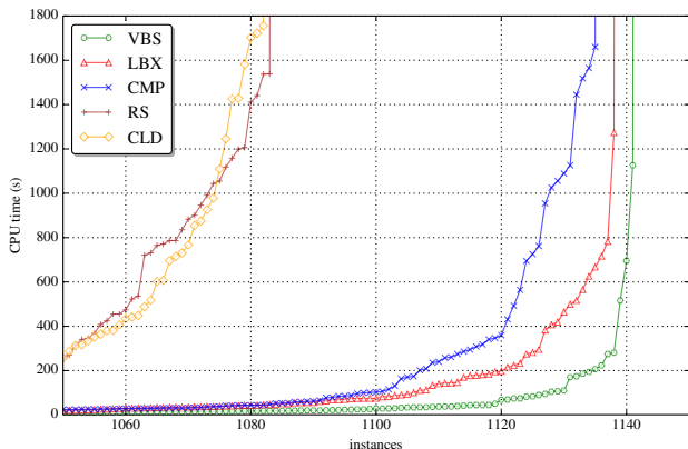
Figure 1: Running times from ijcai13 and mus instances. Note that the plot is zoomed into the range [1050, 1150]
