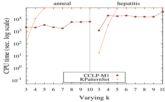
(c) Maximizing the description size.
