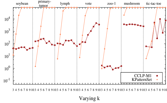
(b) Minimizing pattern diversity.
