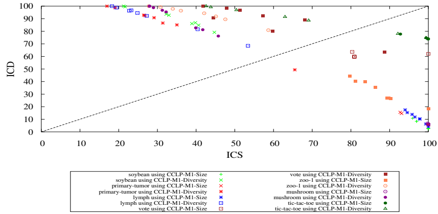
(a) CCLP-M1: Diversity vs. Description size.
