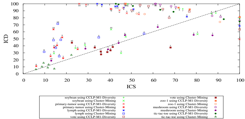
(b) CCLP-M1 with Diversity vs. Cluster Mining (CM).
