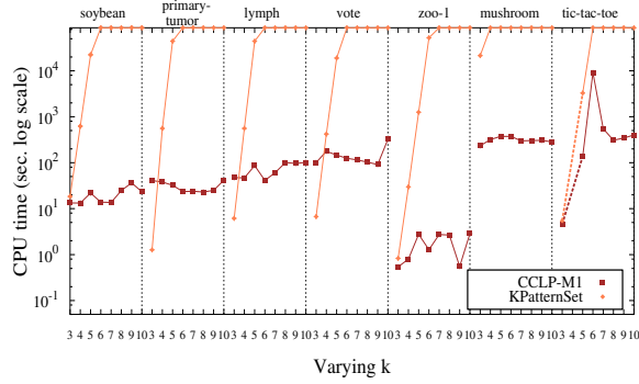
(a) Maximizing description size.
