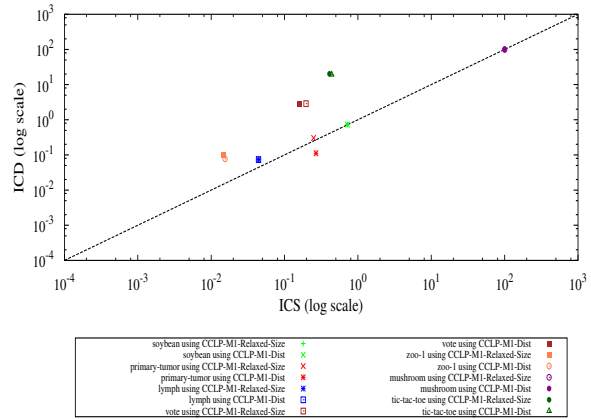
(d) CCLP-M1-relaxed with Size vs. CCLP-M1-Dist.
