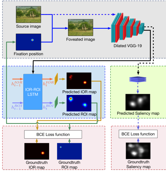
Figure 1: Architecture of the proposed scanpath prediction model, which includes three major components: an image feature extractor (light gray), the IOR-ROI LSTM module (light blue), and the saliency guidance network (light green).
