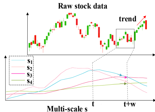
Figure 1: Intuitionistic view of multi-scale patterns within a stock data.
