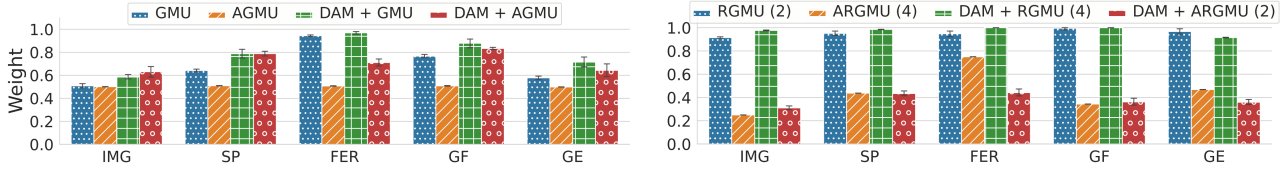
Figure 4: Aggregated modality weights of static (left) and sequential (right) fusion methods. Context sizes are shown within parentheses.
