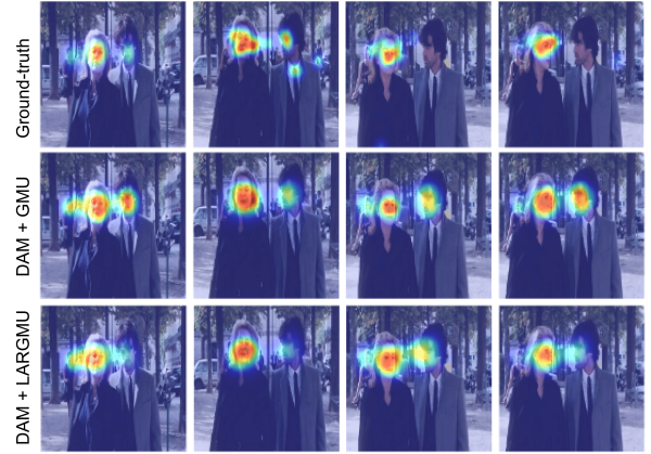
Figure 1: Frame predictions on the Coutrot Database 1 [Coutrot and Guyader, 2014]. DAM + GMU: Directed Attention Module followed by the Gated Multimodal Unit for static integration (middle); DAM + LARGMU: Directed Attention Module followed by the Late Attentive Recurrent GMU for sequential integration (bottom).
