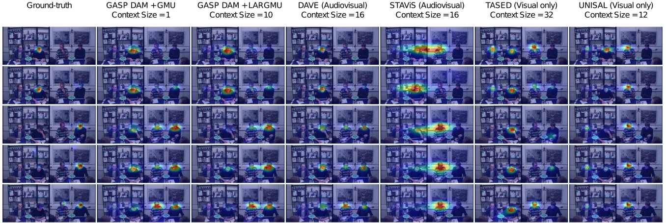
Figure 5: State-of-the-art model comparison on a Coutrot Database 2 [Coutrot and Guyader, 2015] sample. Our sequential (Context Size = 10) and static (Context Size = 1) GASP models employ the audiovisual DAVE (Context Size = 16) as the SCD stage saliency predictor.
