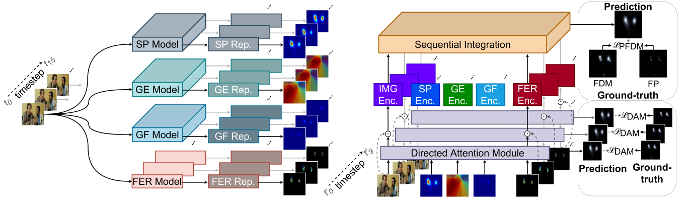
Figure 2: Overview of our sequential two-stage model. SCD (left) extracts and transforms social cue features to spatiotemporal representations. GASP (right) acquires the representations and integrates features from the different modalities.
