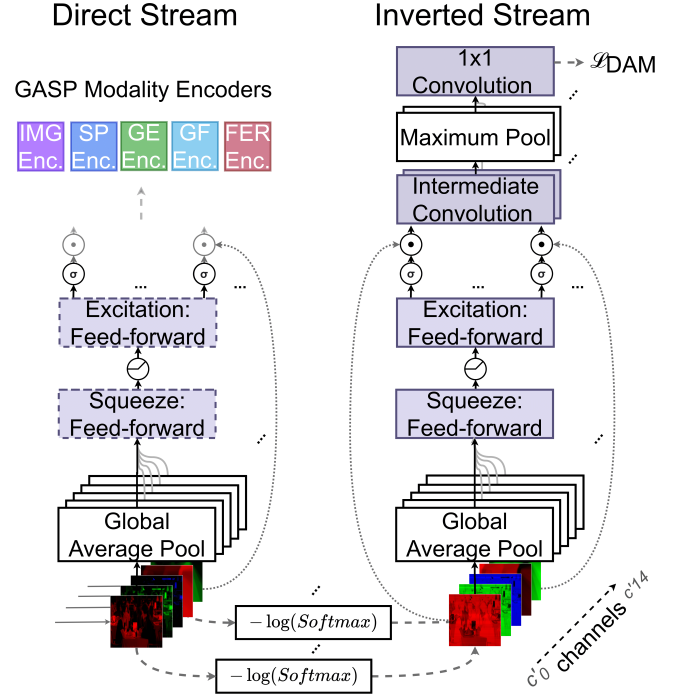
Figure 3: The direct (left) and inverted (right) streams of our Directed Attention Module (DAM). The parameters of the direct stream are frozen and tied to the inverted stream as indicated by the dashed borders.
