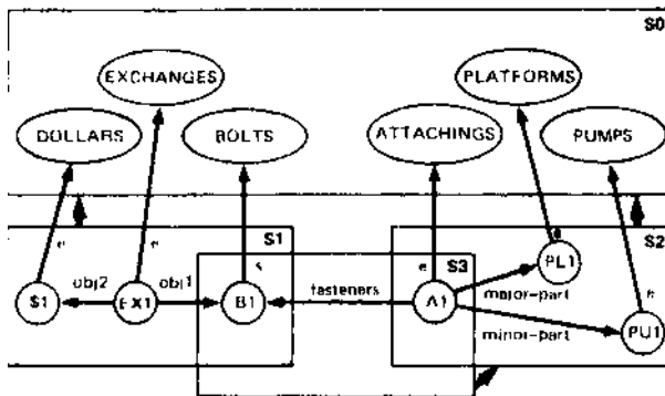
FIGURE 1 A SAMPLE PARTITIONED SEMANTIC NETWORK
