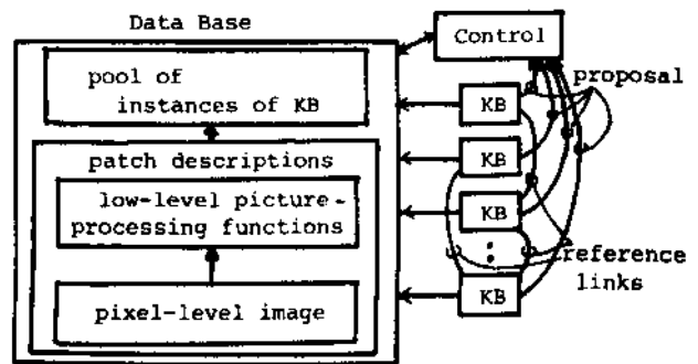
Fig. 3 Concept of Control Structure for Knowledge Block Representations
