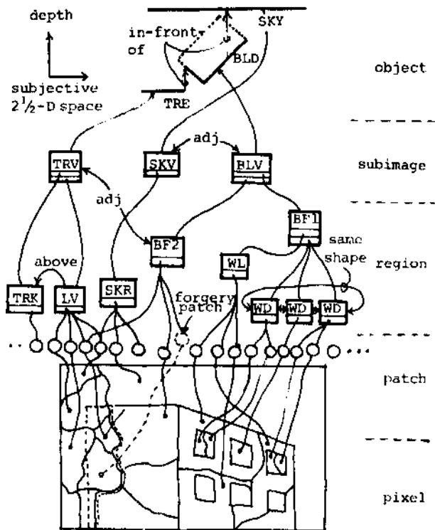
Fig. 1 Illustration of Levels of Description in Processing-Unit Hierarchy
