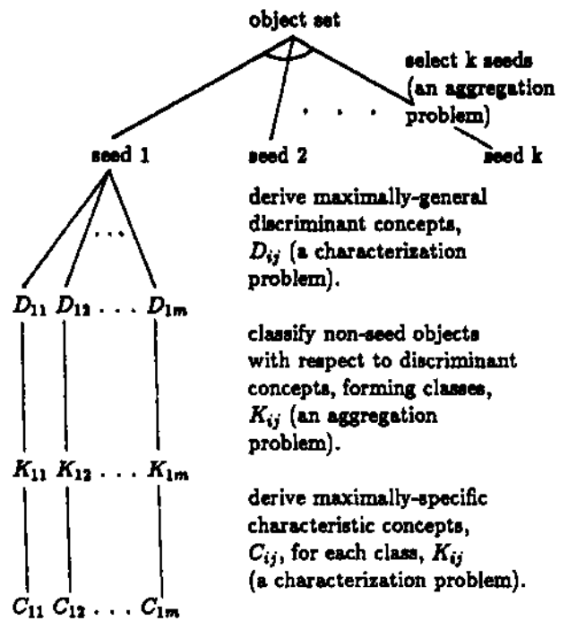
Figure 2 - Aggregation and characterization in the Partitioning Module of CLUSTER/2
