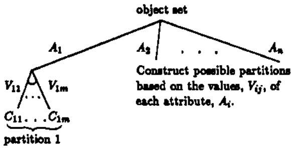
Figure 1 - Aggregation in RUMMAGE and DISCON
