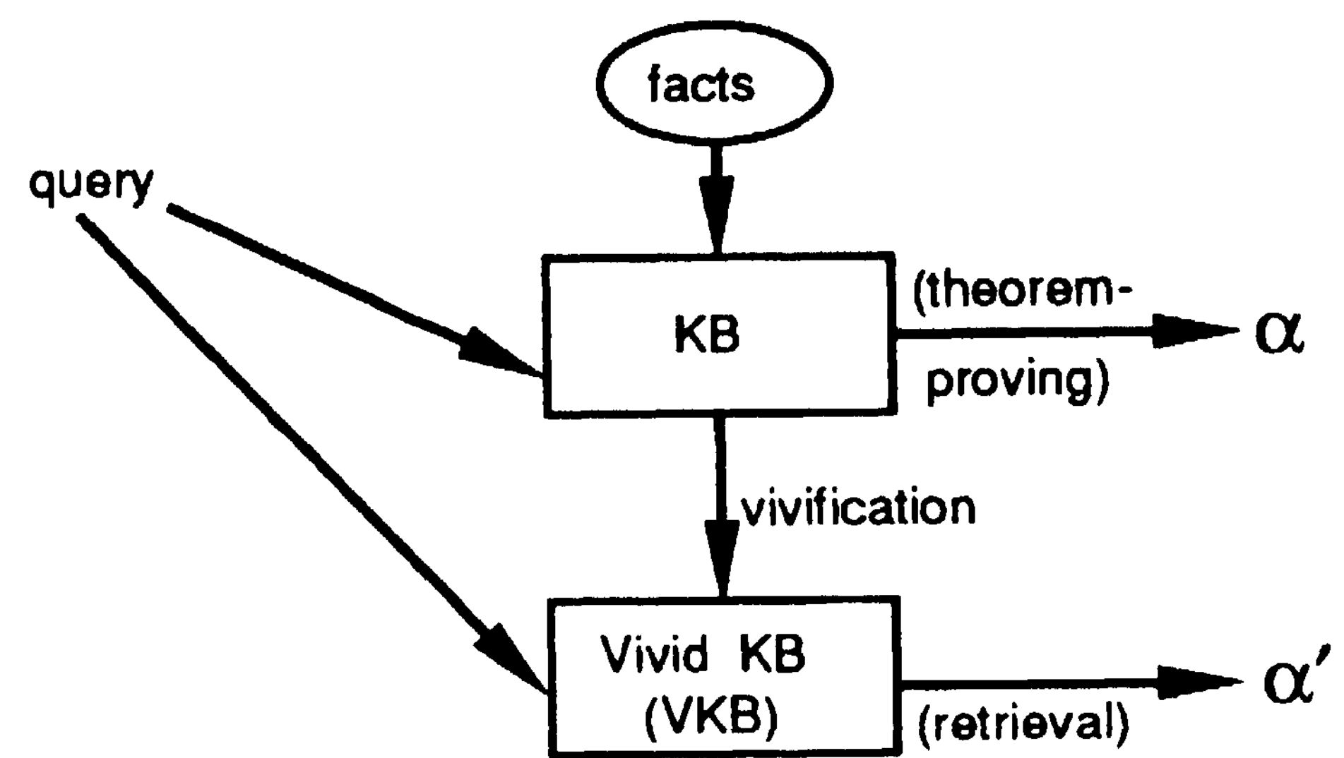
Figure 1: Simple view of a vivid knowledge base.
