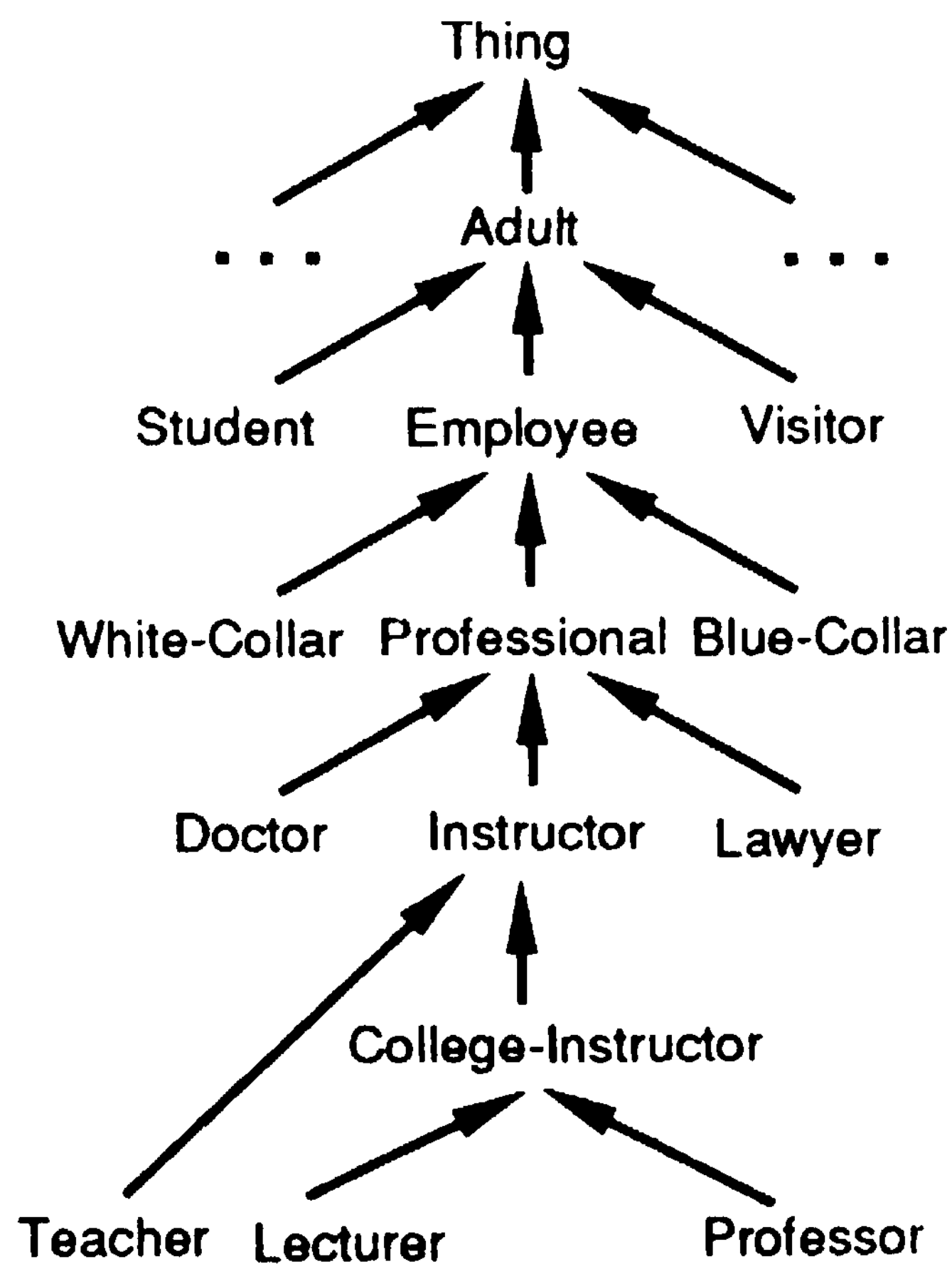
Figure 4: Fragment of a subsumption hierarchy.
