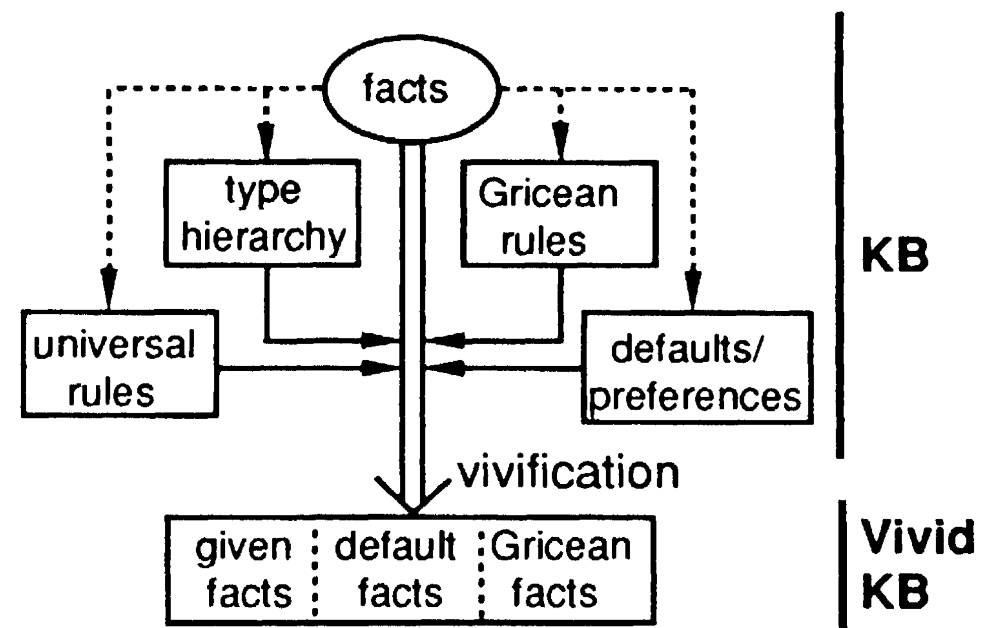
Figure 2: A more general architecture.
