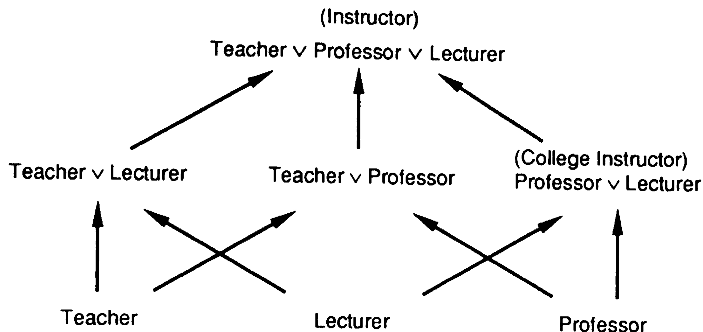
Figure 3: Complete structure for \{Teacher, Lecturer, Professor\} .
