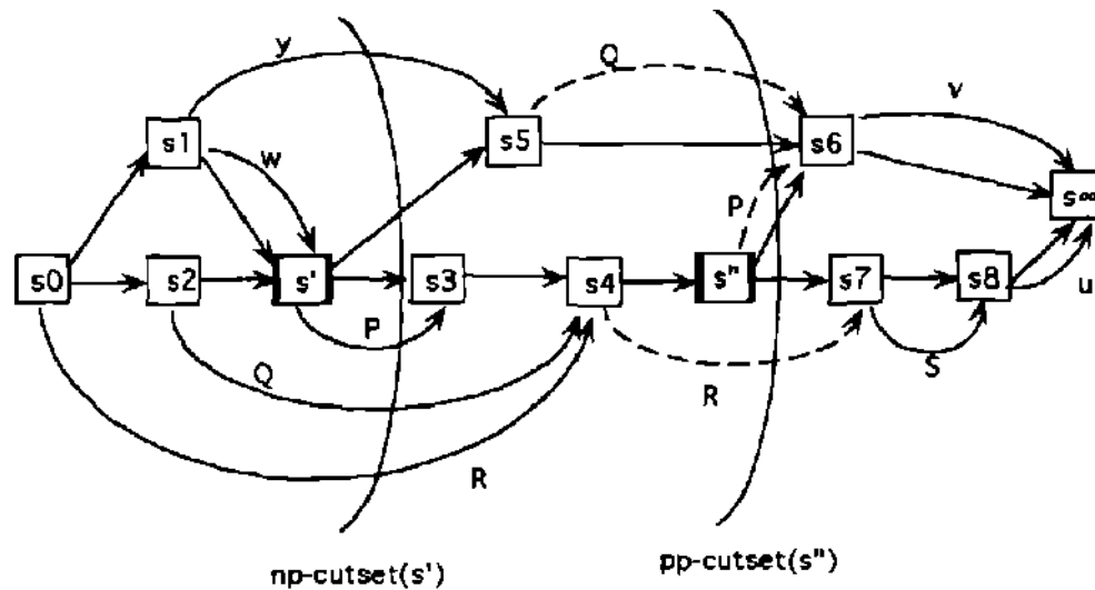
Figure 1 Example illustrating the operation of Cutset-prune strategy. Orderings are shown by straight lines with arrows while the causal links are represented by curved lines with the condition of the causal link shown explicitly near the link. We assume that there are no open conditions corresponding to steps s_5, s_6, s_7, s_8 and s_{\infty} .
