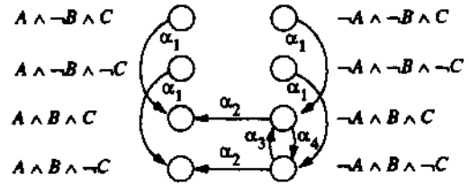
Figure 1: Model for the case in which there are three fluents \mathcal{X} = \{A, B, C\} and four actions: \alpha_1 = \{\neg B \rightarrow B\} , \alpha_2 = \{B \rightarrow A\} , \alpha_3 = \{\neg A \wedge B \wedge C \rightarrow \neg C\} , and \alpha_4 = \{\neg A \wedge B \wedge \neg C \rightarrow C\} .
