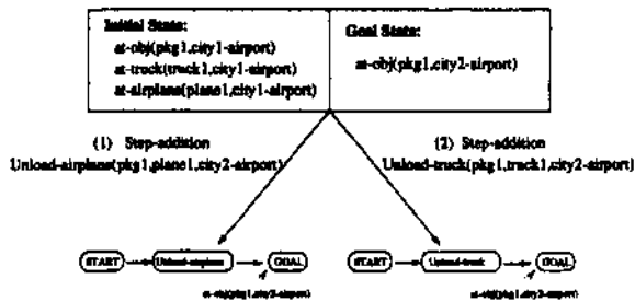
Figure 1: Two refinement candidates for achieving the goal at-obj(pkg1,airport2).
