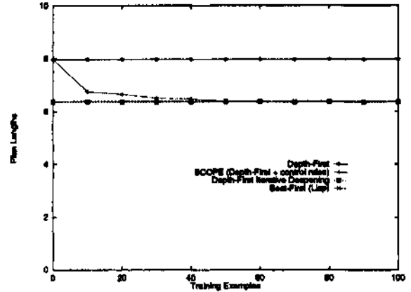
Figure 5: Quality Performance. Here, depth-first iterative deepening and best-first have almost identical performances.
