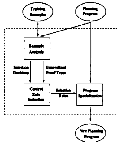
Figure 2: SCOPE'S High-Level Architecture
