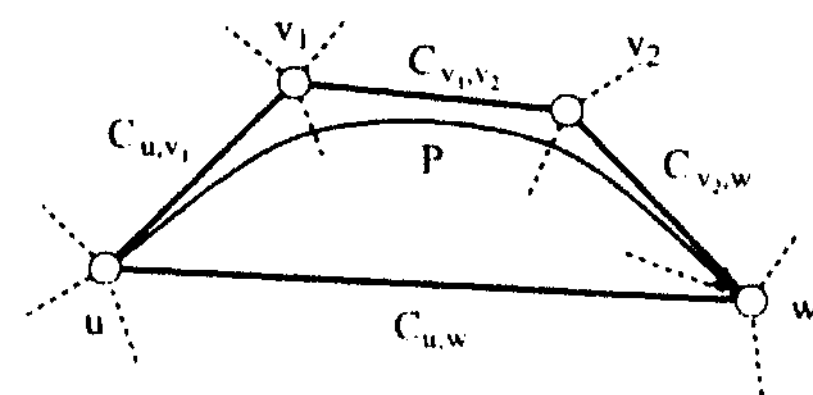
Figure 1: Path Consistency
