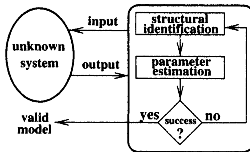
Figure 1: The system identification process
