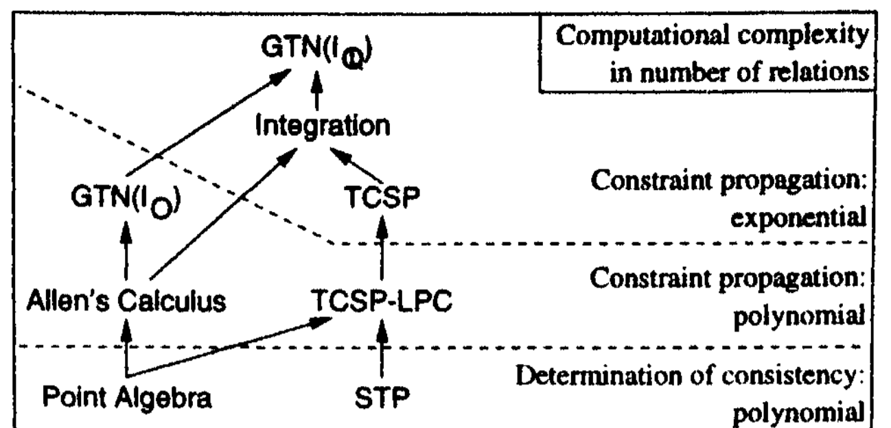
Figure 1: Expressiveness of Reasoning Schemes
