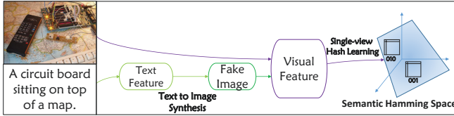
(b) TUCH Framework
