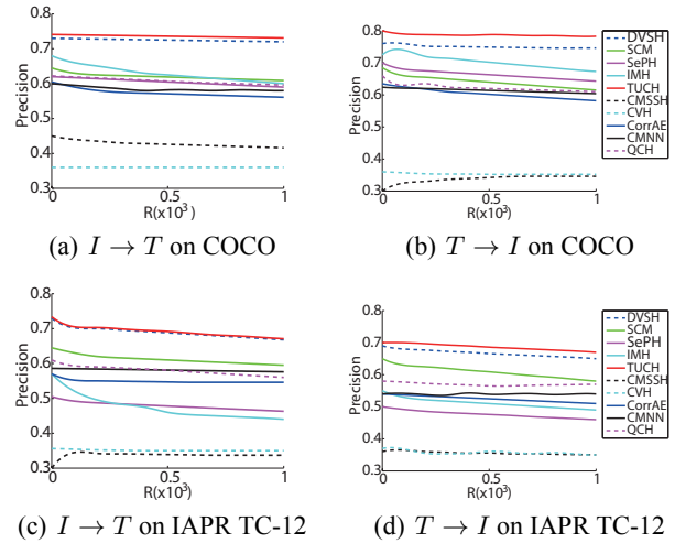
Figure 4: Precision@top-R curves of cross-modal retrieval on Microsoft COCO and IAPR TC-12 @ 32 bits.
