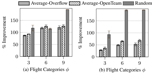
Figure 1: Utility improvement over averaged sample and random uniform in (a) worst case and (b) average case.
