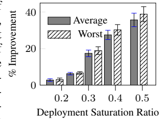
Figure 3: Utility improvement using adaptive decision rules.
