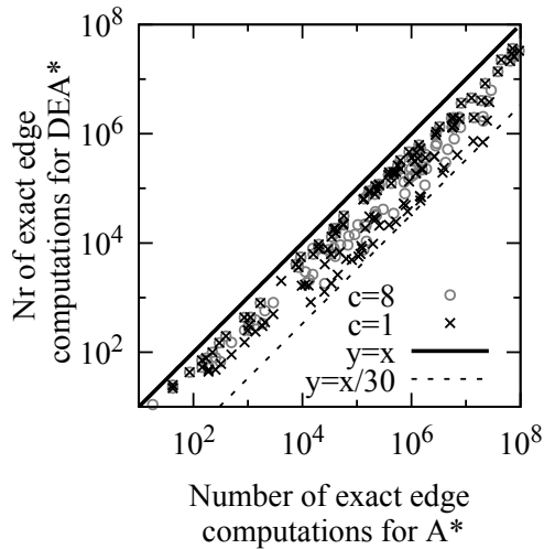
Figure 4: DEA* vs A* in domain independent planning.
