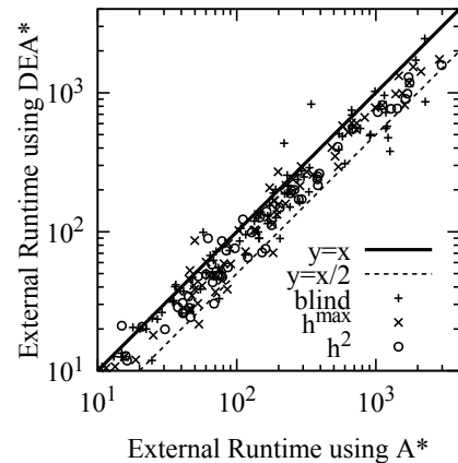
Figure 3: Comparison of the runtime spent for the external calls to DIJA on instances solved by both A* and DEA*.
