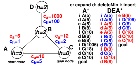
Figure 1: Example illustrating that standard A* computes an unnecessary actual edge cost of BD ( c_a = 1000 ).
