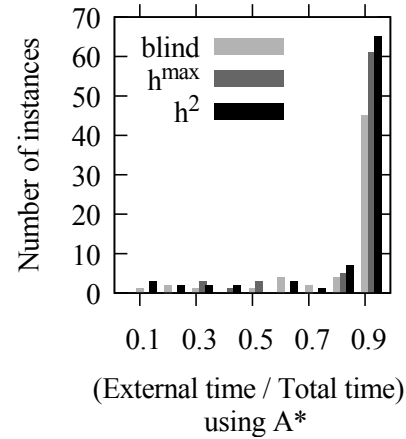
Figure 2: Histogram of the ratio of the external DIJA runtime to the total runtime in A*.
