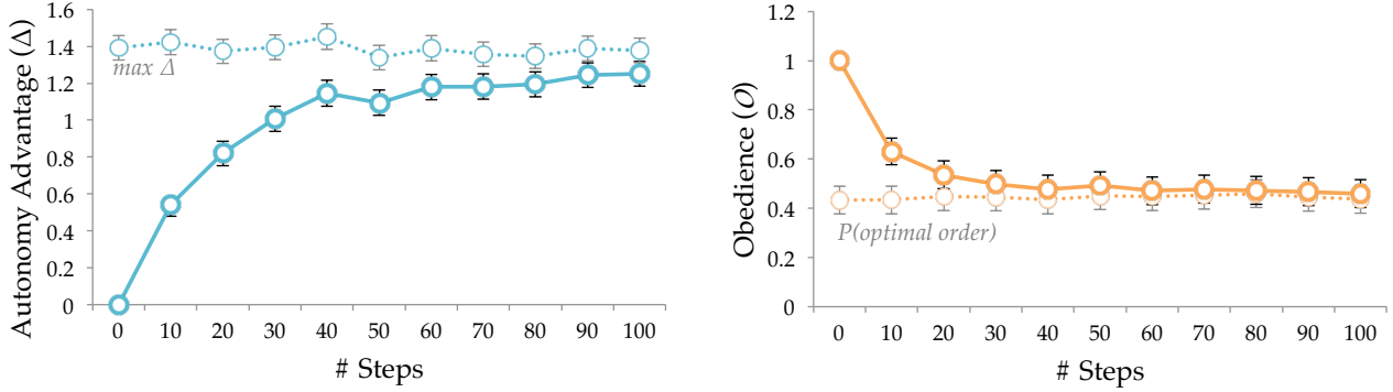
Figure 2: Autonomy advantage \Delta (left) and obedience \mathcal{O} (right) over time.
