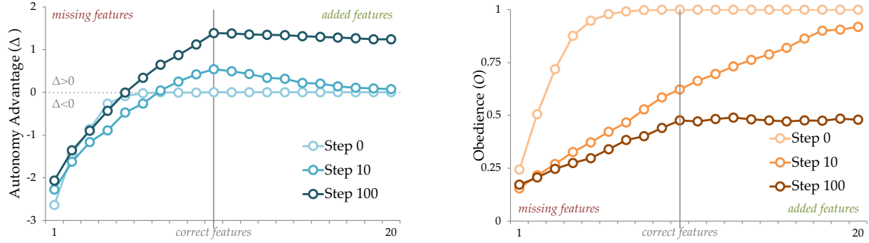
Figure 4: \Delta and \mathcal{O} when \Theta is misspecified
