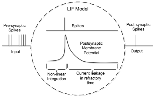
Figure 1: The LIF neuron with discontinuous spikes
