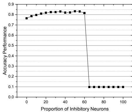
Figure 5: The test accuracy on different proportion of inhibitory neurons
