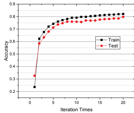
Figure 3: The training and test accuracy with MP balanced tuning
