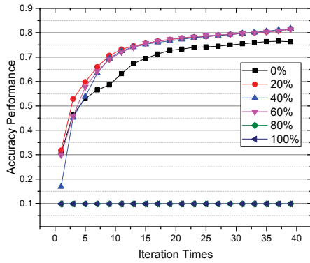
Figure 4: The test accuracy of E-I based balance tuning
