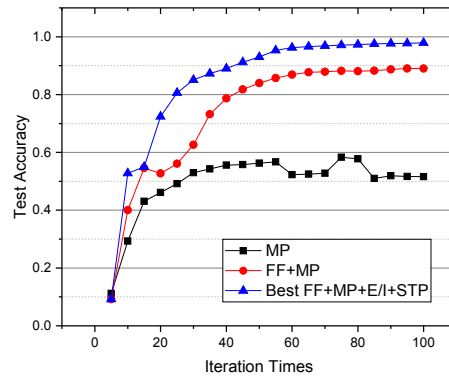
Figure 7: The test accuracy of balanced SNNs with the integration of different rules
