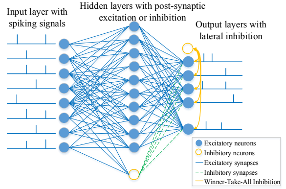
Figure 2: The architecture of a feed forward multi-layered Balanced SNN
