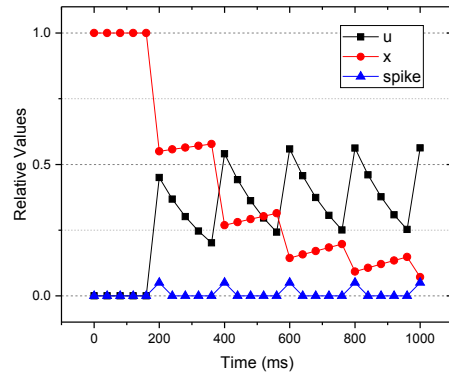
Figure 6: The dynamic variables of u and x with input spikes
