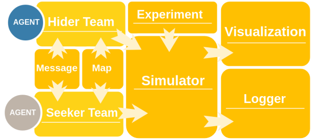
Figure 2: Architecture of Medusa
