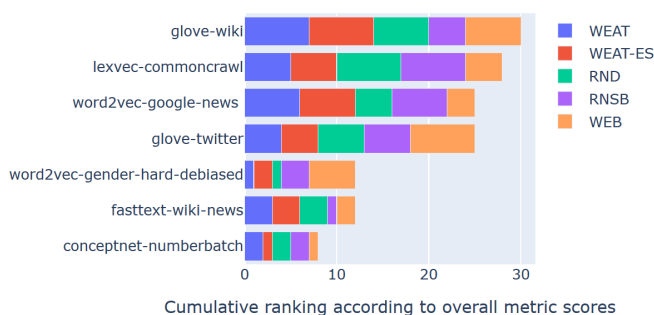
Figure 2: Accumulated rankings for the overall results plus WEB.
