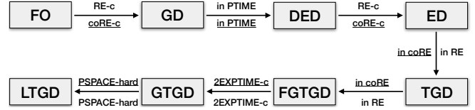
Figure 2: Complexity of Rewritability
