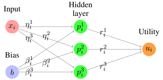
Figure 2: A utility module with 3 hidden nodes ( p = 3 ).
