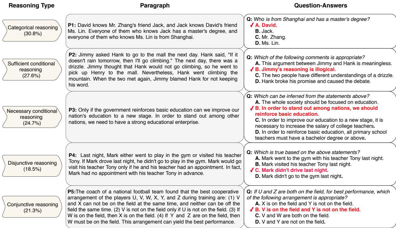
Figure 2: Examples of each type of logical reasoning in LogiQA. (✓ indicates the correct answer.)
