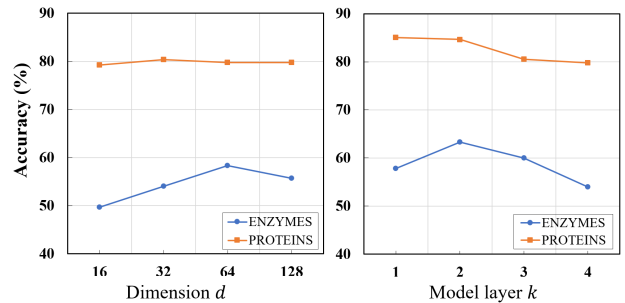
Figure 4: Classification accuracy curve on ENZYMNES and PROTEINS datasets with different values of d and k .
