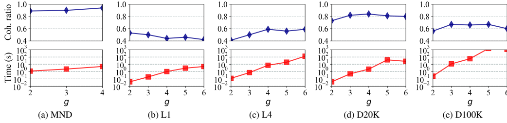
Figure 2: Mean cohesiveness ratio and run time of B 3 F ( \alpha = 0.3 ) under different values of g .
