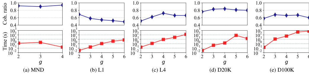
Figure 3: Mean cohesiveness ratio and run time of B 3 F ( \alpha = 0.7 ) under different values of g .
