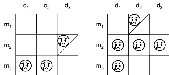
Figure 1: If baby cries under action profile (m_2, d_3) in the left game, the mom is blamable for baby crying. Under the same action profile in the right game, she sees to it that baby cries.
