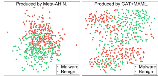
Figure 2: Embedding visualization of malicious/benign repositories.
