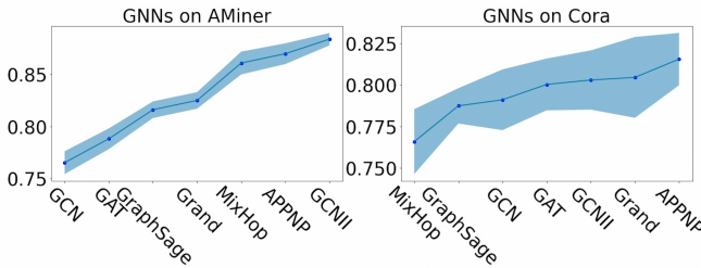
Figure 3: Accuracy of GNNs on AMiner and Cora. The blue area is the fluctuation range of the test accuracy. The vertical axis means the average accuracy based on 100 runs on AMiner’s subgraphs or Cora’s random splits.
