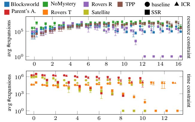
Figure 4: Comparison of average number of expansions over commonly solved task. Error bars represent the 95% confidence intervals. top: resource constraint domains, x value corresponds init_\rho ; bottom: time constraint domains, x value corresponds to size difference of the relaxed time window to the original one.
