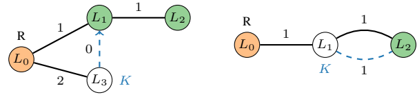
Figure 3: left: Map of separation of ICR and SSR from baseline, initial location: L_0 , goal: visit L_1 and L_2 . right: Map of separation of ICR from SSR, initial location L_0 , goal: visit L_2 .
