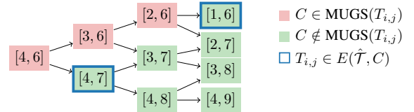
Figure 2: Part of hasse diagram for the time relaxed tasks of the running example. [i_1, j_1] \rightarrow [i_2, j_2] means T_{i_1, j_1} \sqsubseteq T_{i_2, j_2} . T_{3,7} \notin E(\hat{T}, C) because T_{4,7} \sqsubset T_{3,7} .
