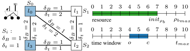
Figure 1: Running Example
